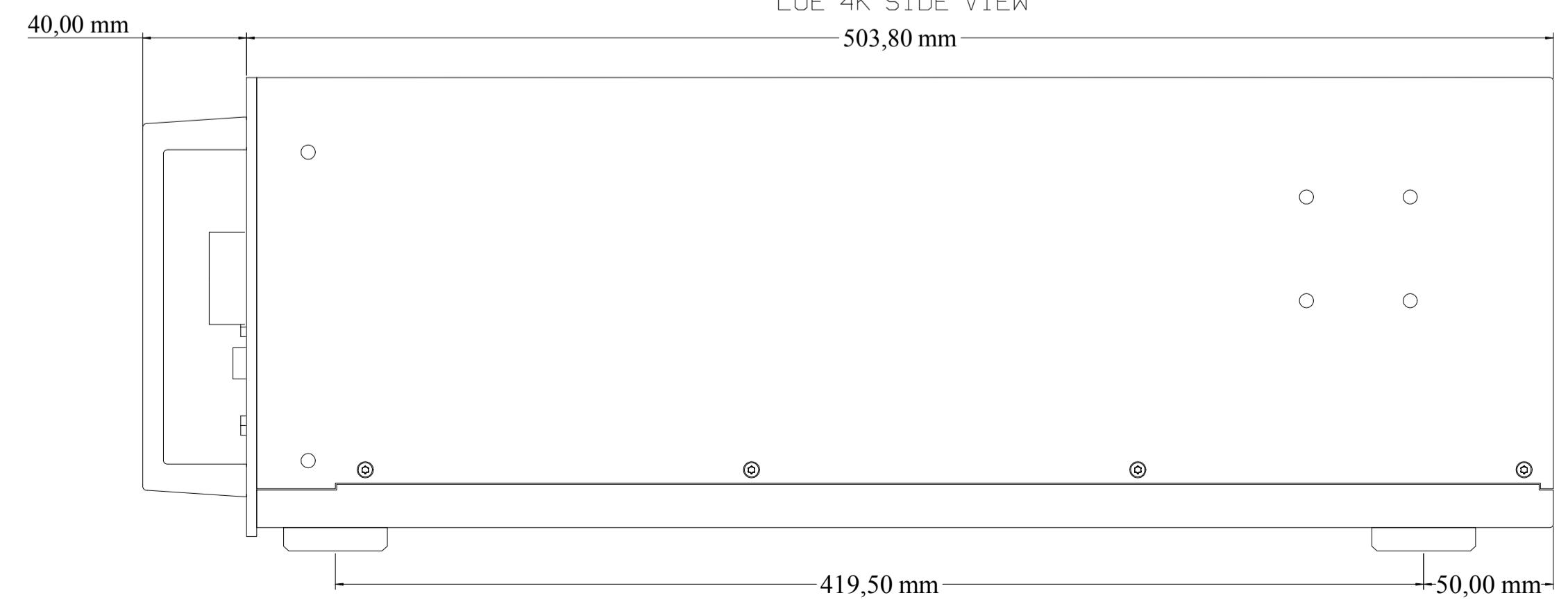
LOE 4K SIDE VIEW
