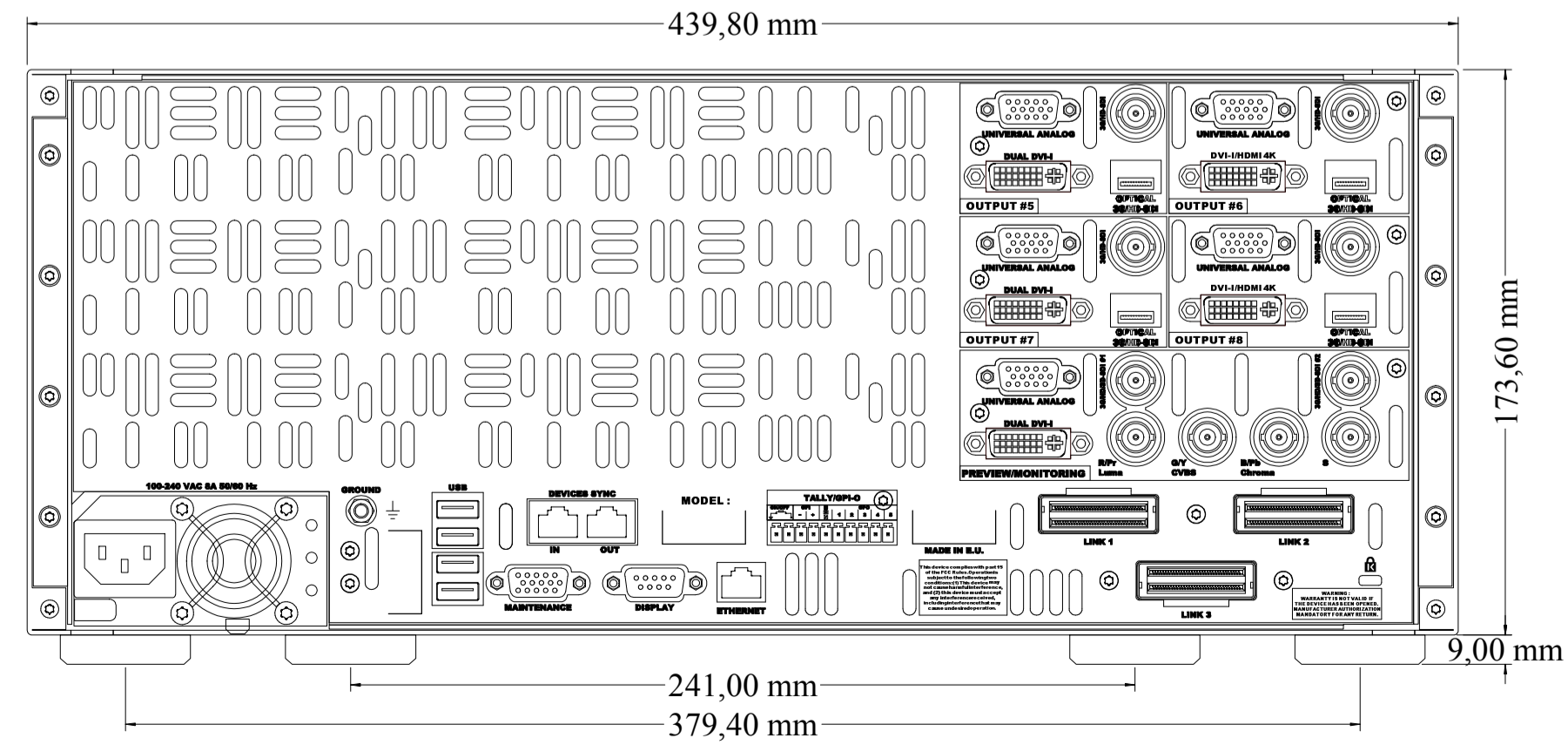
LOE 4K REAR VIEW
